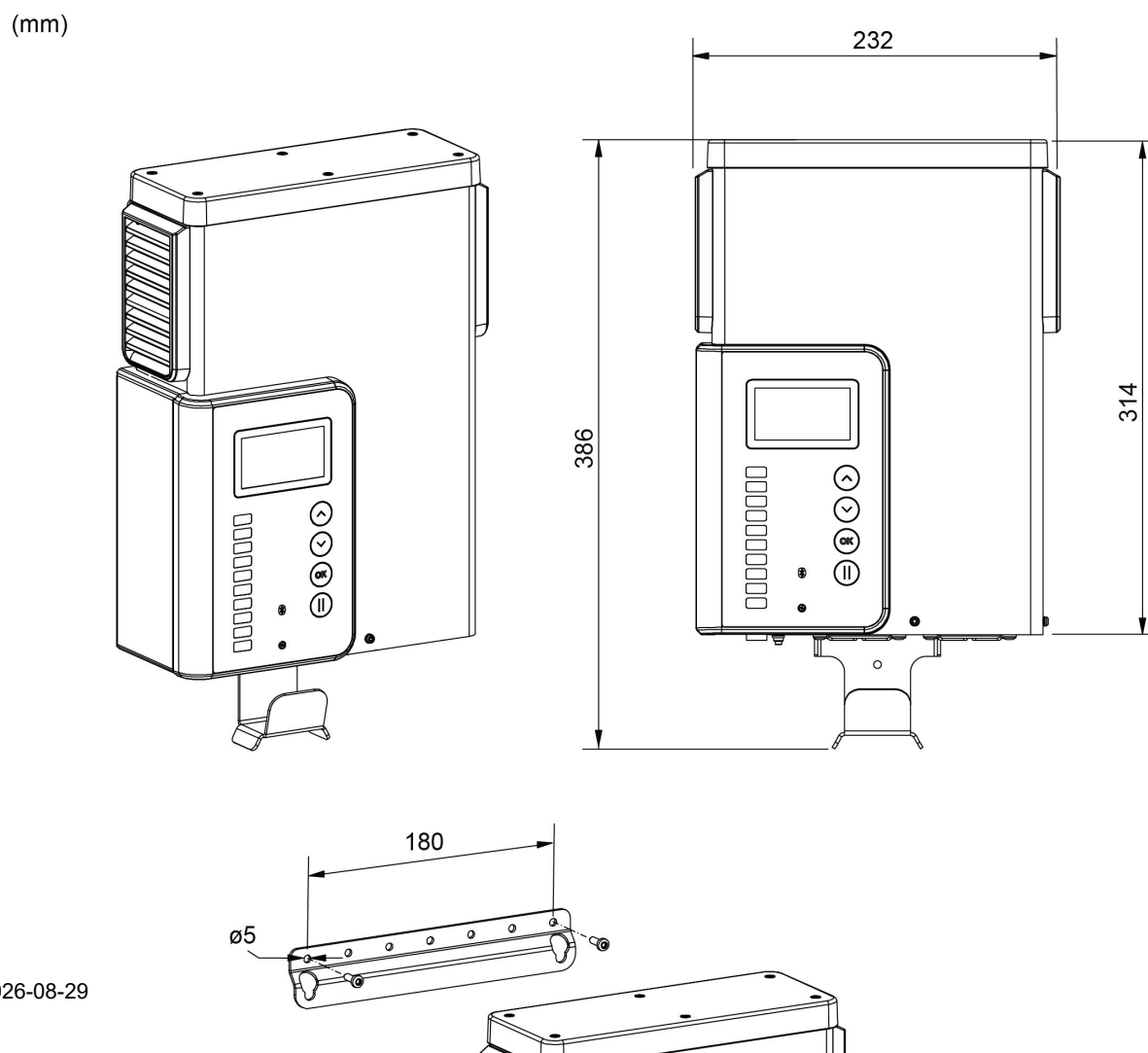
Fig. 5 Installation options
