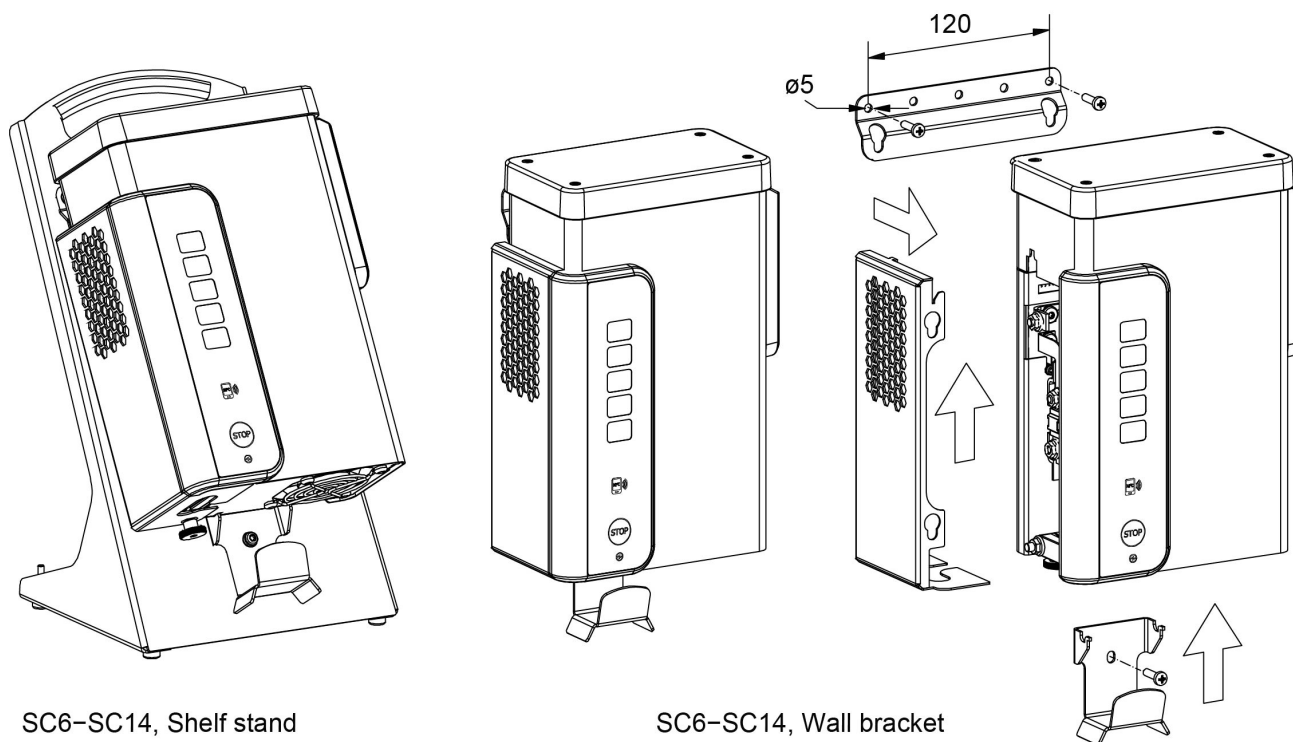
Fig. 5 Installation options
